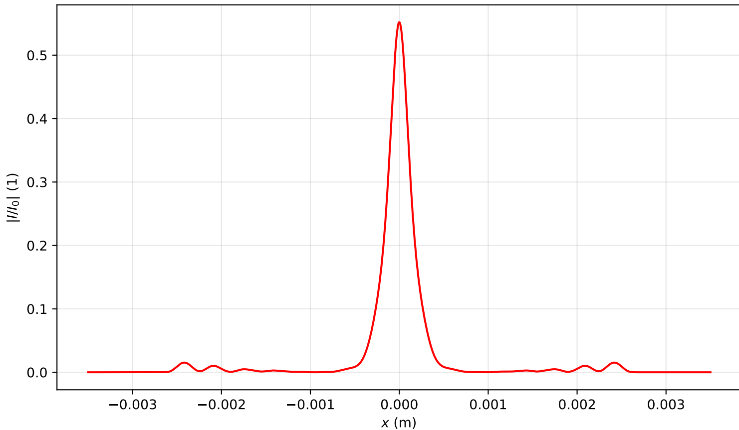
Intensity profile I(x, y = 0, z = 2.229)/I_0 , \text{Pin}=7.0\text{Pcr} , artificial time
